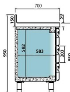
BMGN 1/3x100
