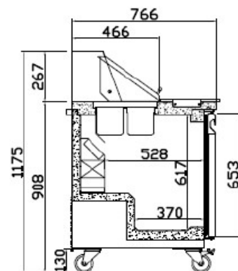
PERFIL/RIGHT VIEW/VUE EN PLAN
