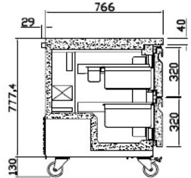
PERFIL/RIGHT VIEW/VUE EN PLAN
